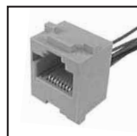
70-511 Modular female chassis jack. 8-position, 8 wires and lugs. For 8 conductor cable equipment.
