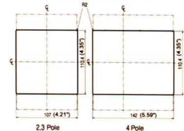
Panel cover cutting size
