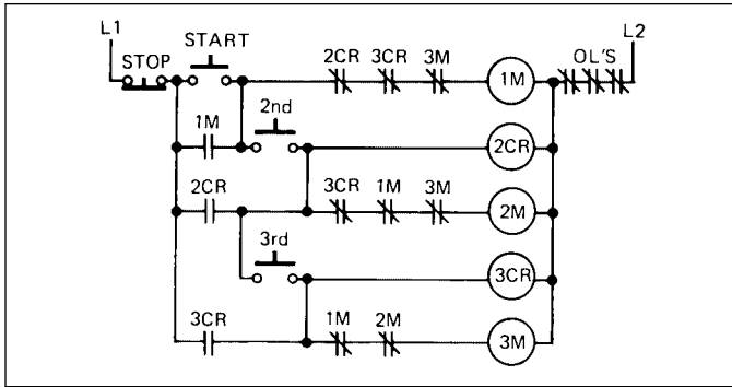
Figure 13 Control for Three Speed with a Compelling Relay to Insure Starting on Low Speed
