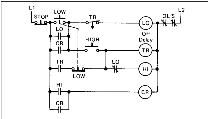
Figure 15 Control for Two Speed to Provide Automatic Deceleration from High to Low Speed
