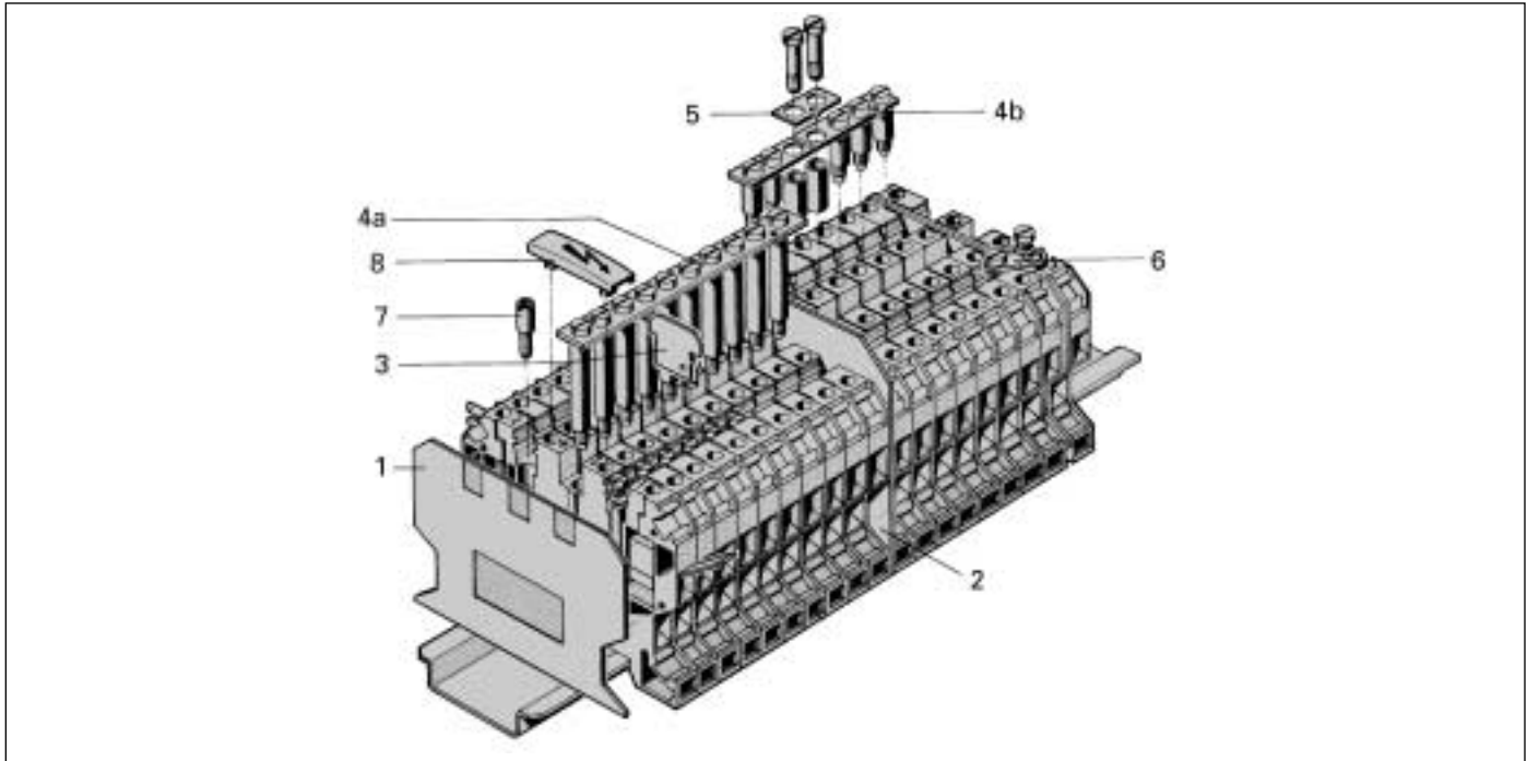
End Plate 8WA1817
