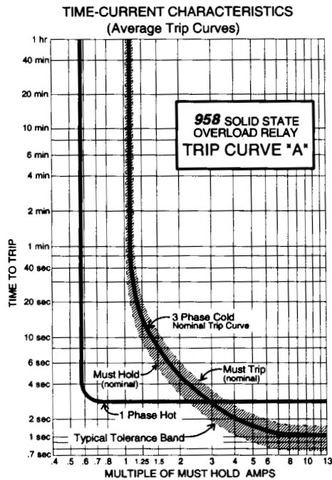
Trip Curve A
