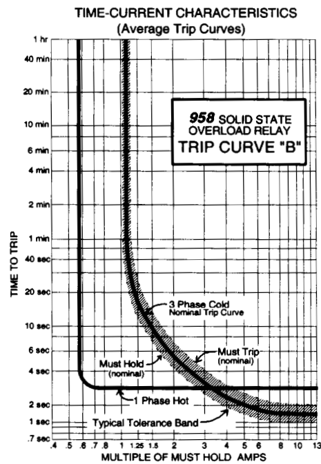
Trip Curve B
